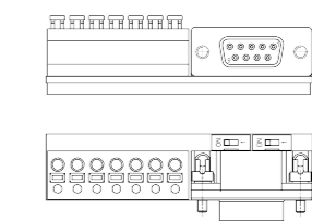
Abb. 4 SPC210-Adapter
